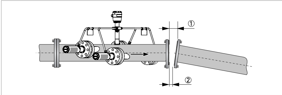
Figure 3-8: Flange deviation
