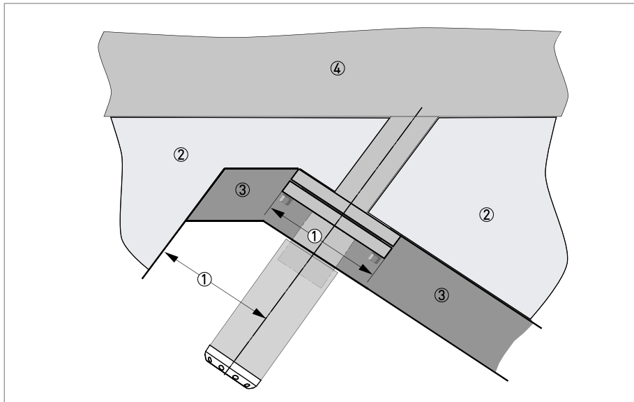
Figure 3-10: Thermal insulation
