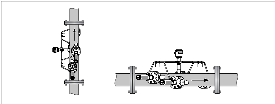
Figure 3-6: Horizontal or vertical installation
