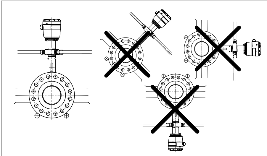
Figure 3-7: Mounting position
