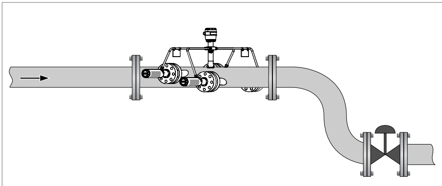
Figure 3-9: Recommended installation of the control valve
